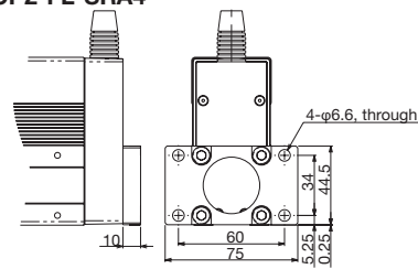
When flange bracket (rear) is mounted
