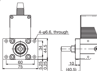
When flange bracket (front) is mounted
