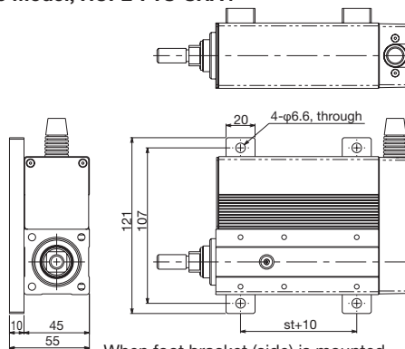
When foot bracket (side) is mounted
