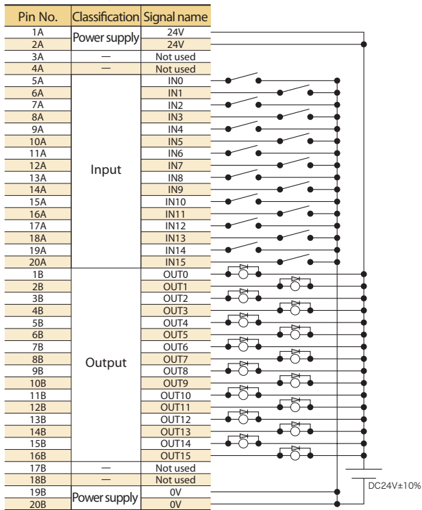
PIO connector (NPN specifications)
