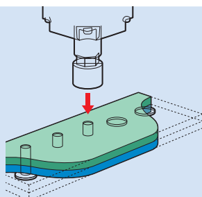
Staking work
