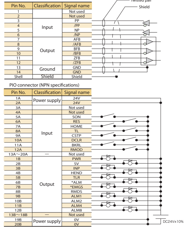
Pulse connector
